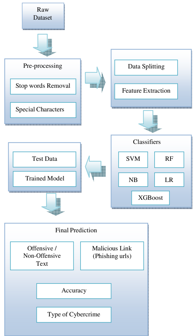
Fig3. Proposed Model
