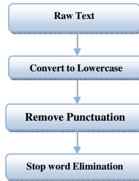
Fig 2 Data Preprocessing
