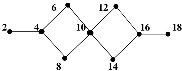
Figure 10: Vertex even mean labeling of 2C_4+2P_2
