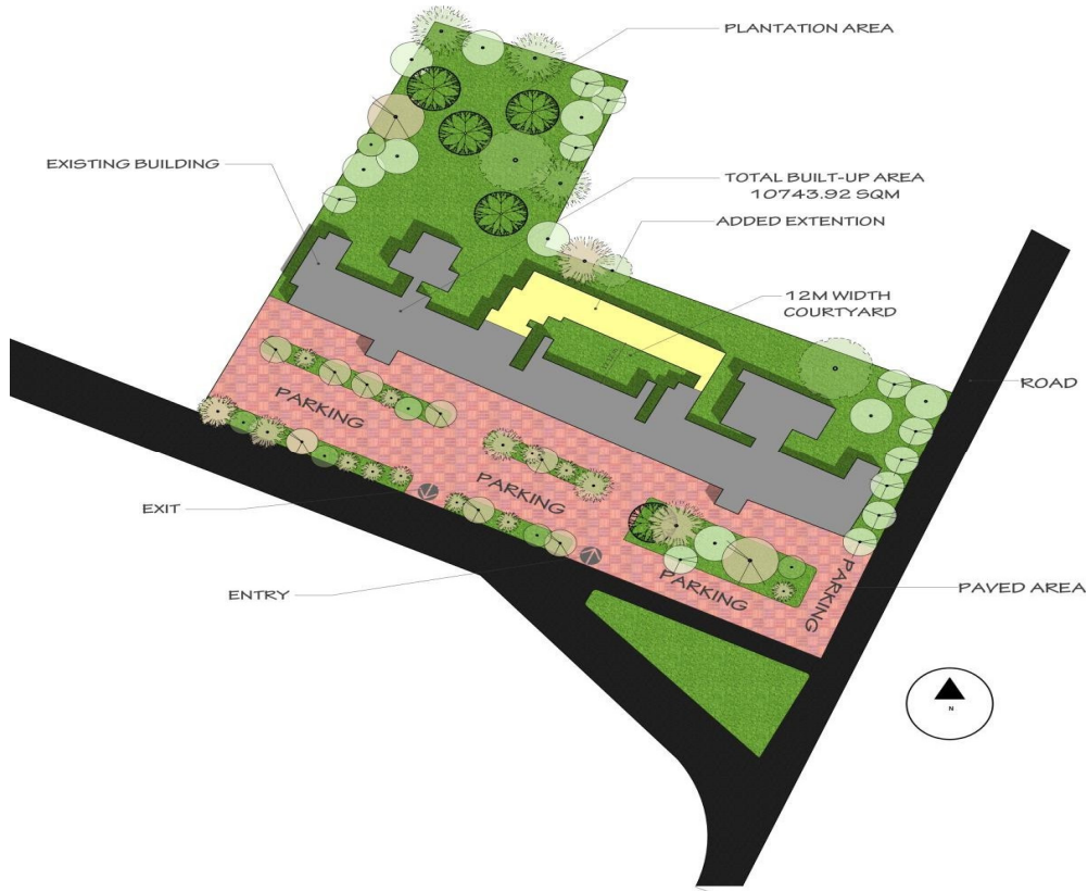
Figure 32. Site plan
