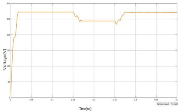
Fig.7. Sag compensation
