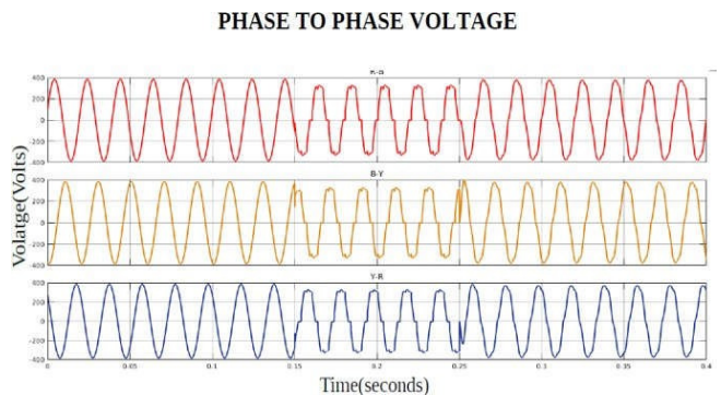
Fig.7. Phase to phase sag voltage
