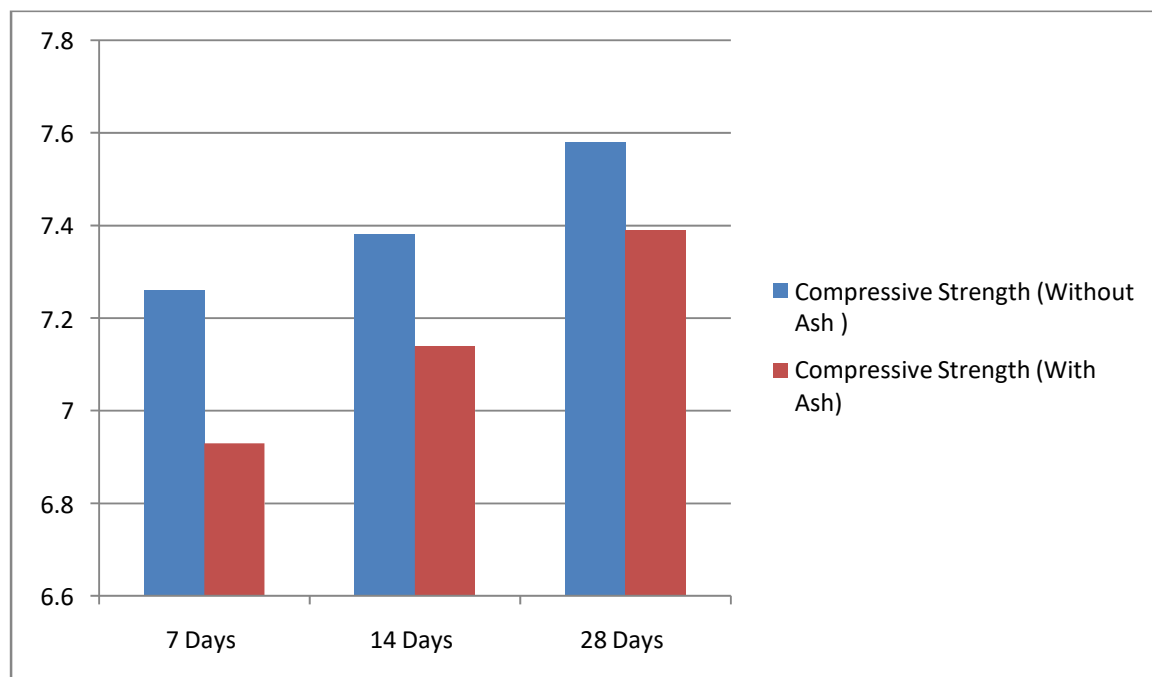
Fig 1:- Compressive Strength of Sample Without Ash & With Ash after 7 Days,14Days,28 Days.
