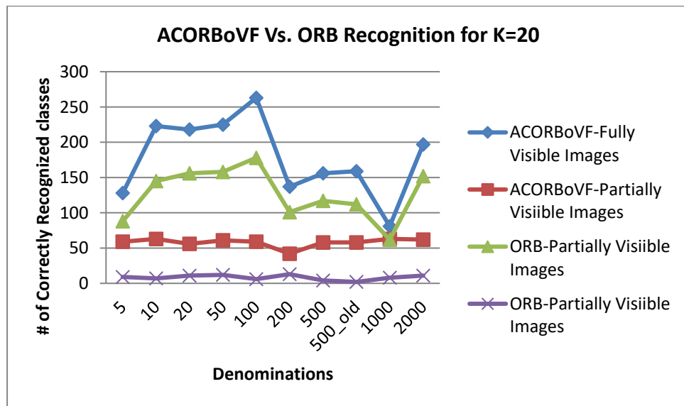
Figure 17. Number of correctly identified images using ACORBOVF and ORB
