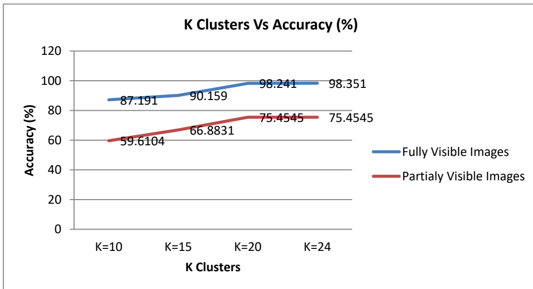
Figure 26. The overall accuracy of the ACORBOVF for different values of K
