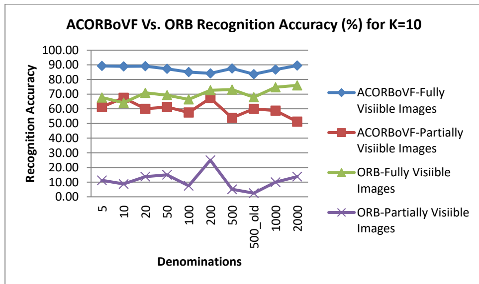
Figure 10. Recognition accuracy of the ACORBoVF and the ORB
