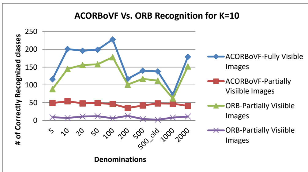
Figure 9. Number of correctly identified images using the ACORBoVF and the ORB
