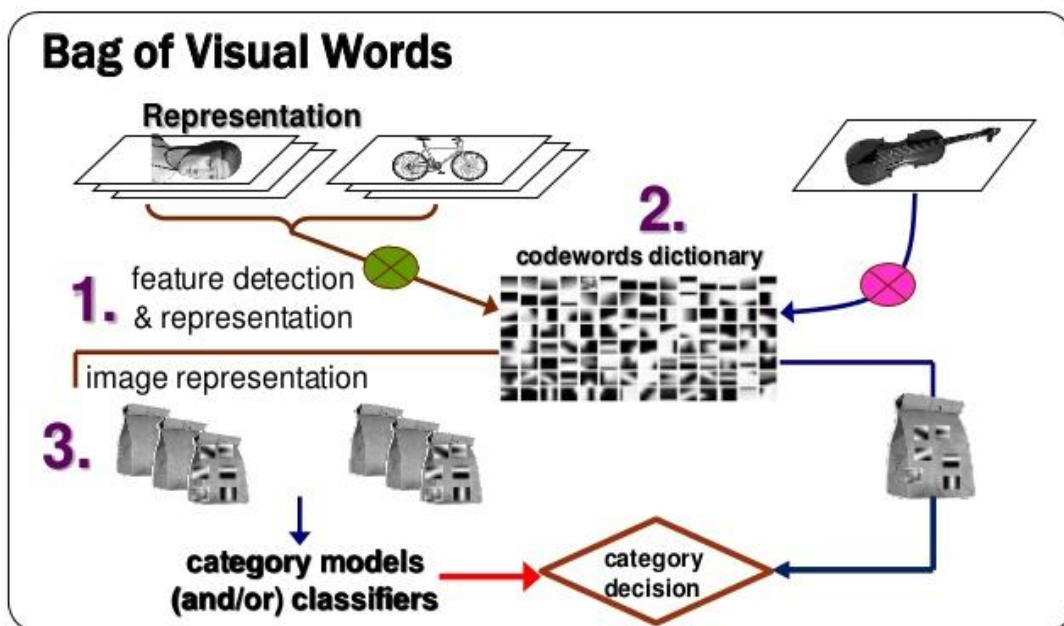
Figure 4. Classification process of visual words model
