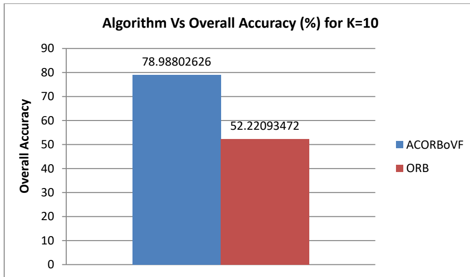
Figure 12. The overall performance of the ACORBoVF and the ORB
