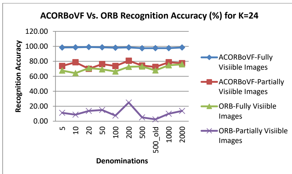
Figure 22. Recognition accuracy of the ACORBOVF and the ORB
