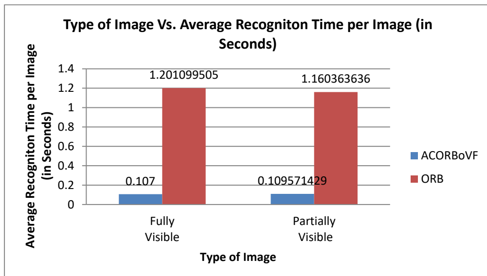
Figure 11. Average time taken per image by the ACORBoVF and the ORB
