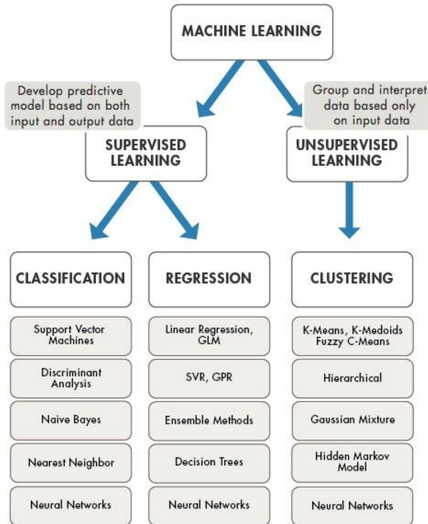
Figure 2. Supervised Vs. Unsupervised Learning
