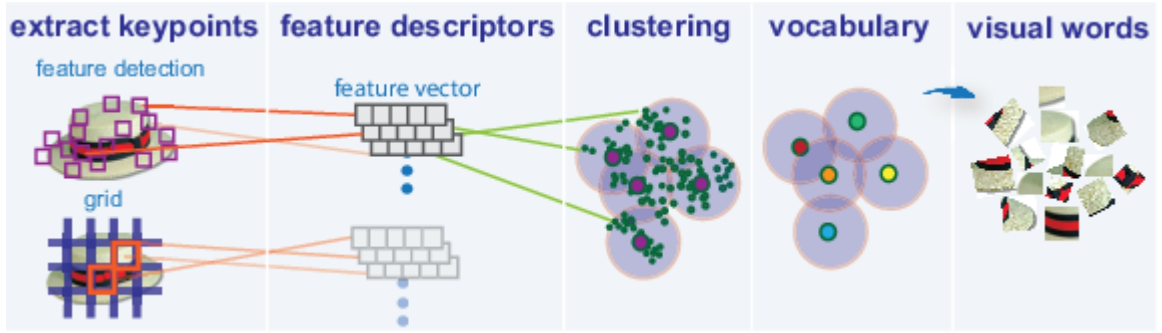
Figure 5. Generating visual vocabulary
