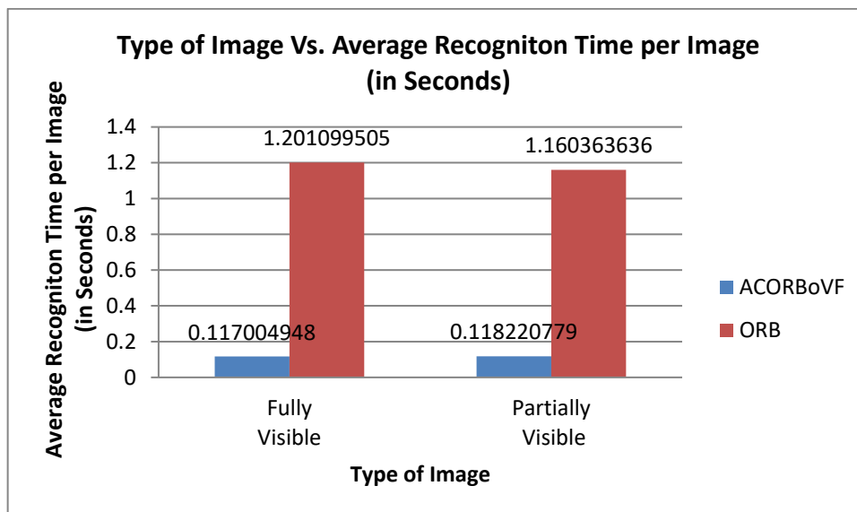
Figure 19. Average time taken per image by the ACORBOVF and the ORB
