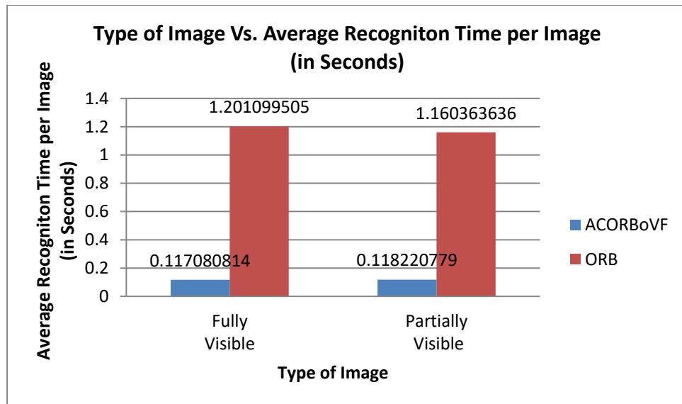
Figure 23. Average time taken per image by the ACORBOVF and the ORB
