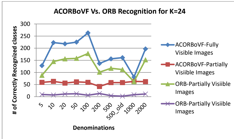
Figure 21. Number of correctly identified images using the ACORBOVF and the ORB
