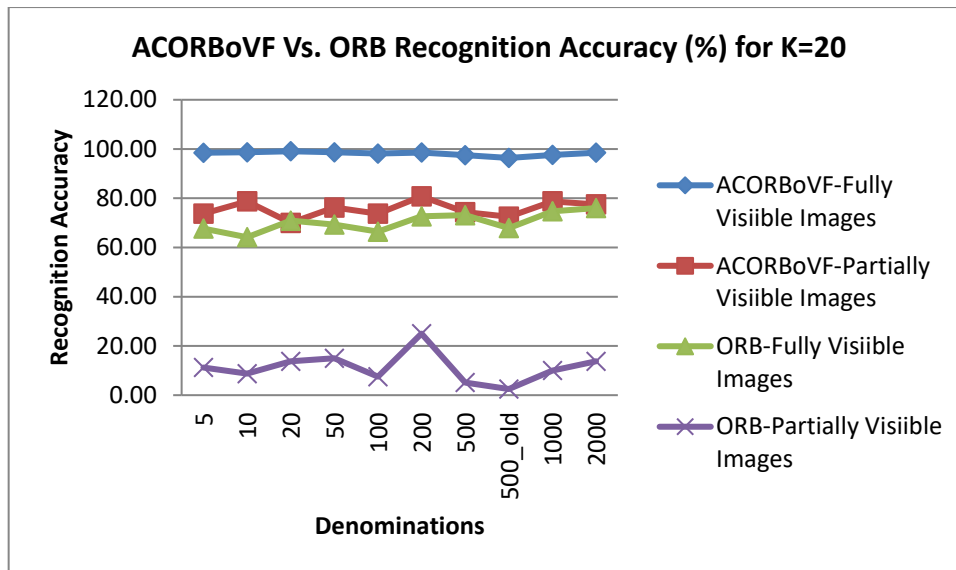
Figure 18. Recognition accuracy of ACORBOVF and ORB
