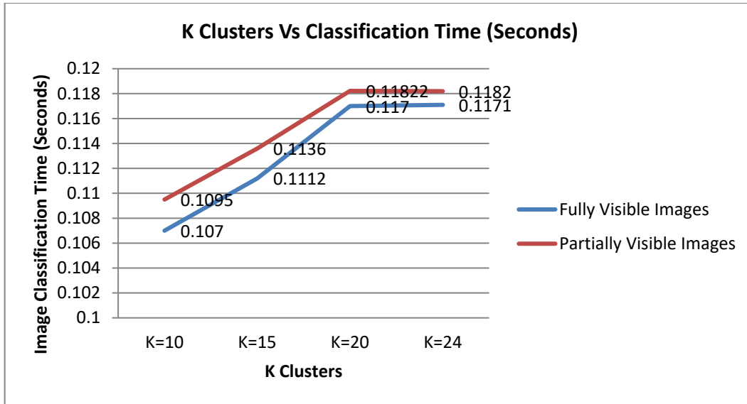
Figure 25. Average time consumption by the ACORBOVF for different values of K
