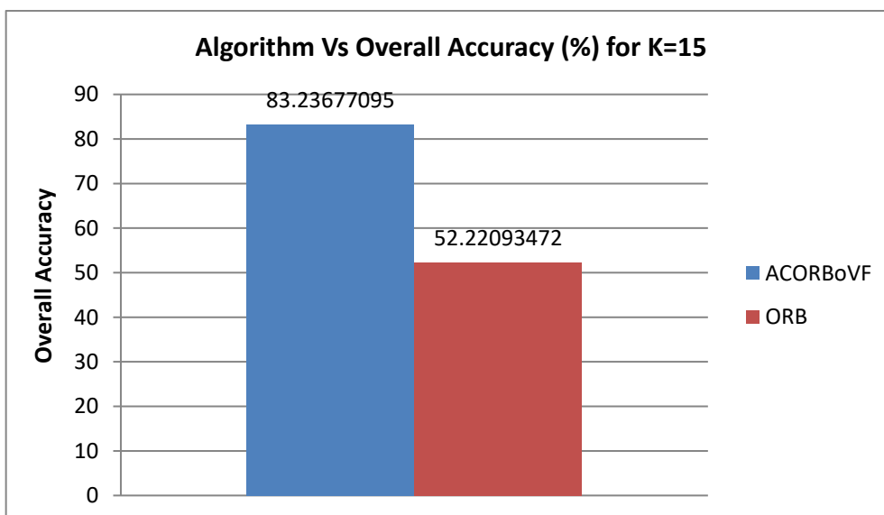
Figure 16. The overall performance of the ACORBOVF and the ORB
