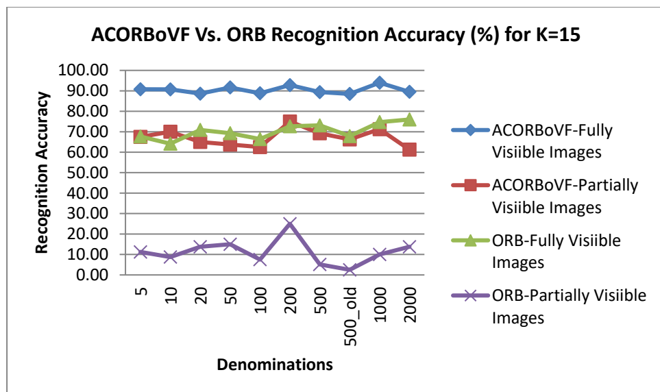
Figure 14. Recognition accuracy of the ACORBOVF and the ORB
