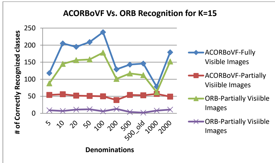
Figure 13. Number of correctly identified images using the ACORBOVF and the ORB
