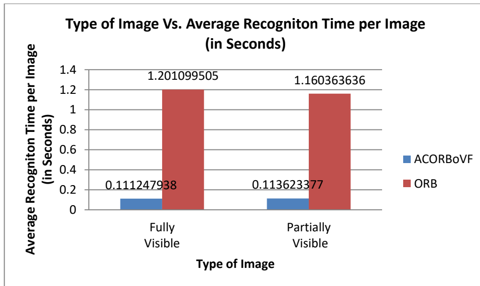
Figure 15. Average time taken per image by the ACORBOVF and the ORB
