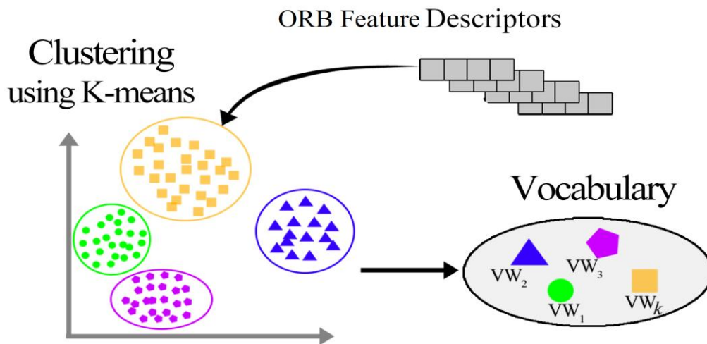
Figure 8. ORB based dictionary vocabulary creation process
